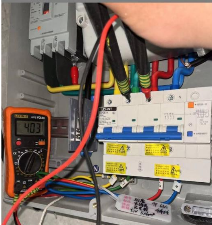
L- L voltage: Three-phase 400V \pm 15\% Single-phase 230V \pm 15\%
